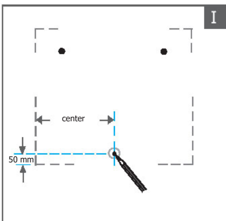
I Mark drill Position for bottom fixing as indicated.
