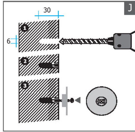
J Drill 6 mm hole 30 mm deep and fix with plugs and screws with small round button facing the wall.
